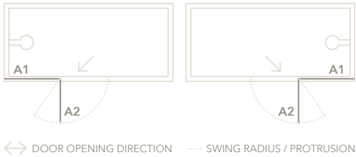
OVERHEAD LAYOUT
